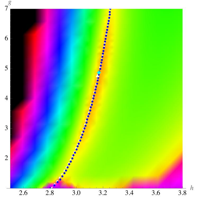
FIG. 4. Heat map of \chi(h, g) given in Eq. (15) for o = 4 , N_m^{\max} = 16 . The white dashed line is the critical line of [1], with a white shamrock marking their sweat spot (best agreement with a CFT). In dark blue dots the minimum of the valley of \chi(h, g) . The cyan diamond marks the global minimum of \chi(h, g) .
