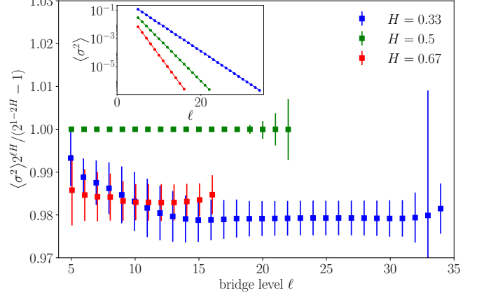
FIG. 10. Ratio between sampled variance and no-neighbour-estimate of variance (cf. Eq. (17)) of an inserted midpoint X_m versus the level of the bisected bridge. For H = 0.5 (green), the ratio equals 1, as BM is Markovian. For H \neq 0.5 , the variance fluctuates, as shown by the error bars for one standard deviation. Numerical errors due to a loss of floating point precision become relevant around L_{\text{max}} \simeq 11/H . ABSec was used with an initial grid \Lambda^8 and \epsilon' = 10^{-9} .
