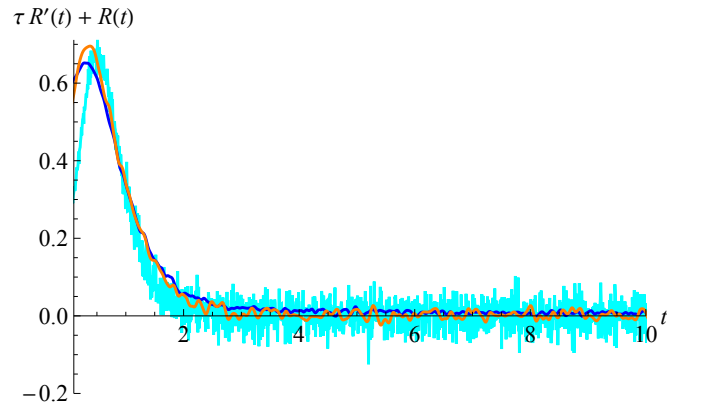
FIG. 10. The function \delta_{\text{BL}}(t) := (\tau \partial_t + 1)R(t) for the measured response function with m^2 = 10^{-2} (blue), m^2 = 10^{-3} (orange), m^2 = 10^{-4} (cyan). Parameters as in Fig. 9. ***plots missing, one could also put \delta_{\text{BL}}(t) on the y-axis.
