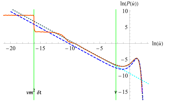
FIG. 7. P(\dot{u}) for m^2 = 10^{-3} , \delta t = 10^{-3} , v = 0.1 , N = 5 \times 10^8 , DNI (orange, solid line). The blue dashed curve is given by Eq. (73), the gray dotted one by the same formula, replacing m^{-2} \rightarrow 0.39m^{-2} , yielding a perfect fit. Cyan dotted is the result for ABBM, Eq. (44).
