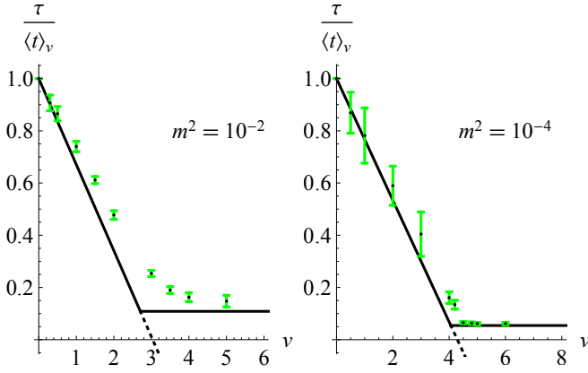
FIG. 11. Inverse of the measured time scale \langle t \rangle_v := \int_0^\infty dt t R_v(t) , as a function of v . The data points are given with 99% confidence intervals (green). Superimposed are the two analytical curves (81), valid for v \leq f_c , and (82), valid for v \geq f_c . DNS, \delta t = 10^{-4} , \delta u = 10^{-6} for m^2 = 0.01 , and \delta u = 10^{-4} for m^2 = 10^{-4} .
