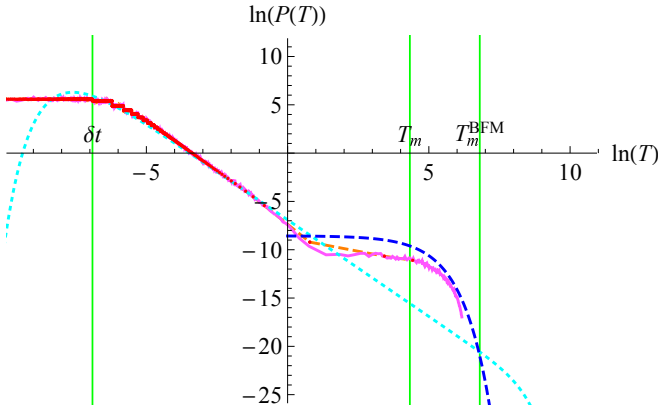
FIG. 14. P(T) measured numerically via INS for m^2 = 10^{-3} , \delta w = 1 , \delta t = 10^{-3} , N = 5 \times 10^8 . This is compared to the theory prediction (48) for ABBM (cyan dotted), and (66) for DPM (blue, dashed).
