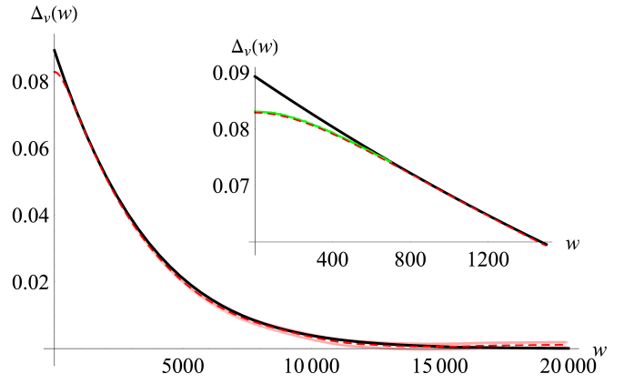
FIG. 18. The numerically measured \Delta_v(w) for v = 0.5 (red, dashed, with 95%-confidence intervals in shaded red) as defined in Eq. (18). For w > 1000 it agrees well with the theoretical prediction (91) (black, solid). The inset shows the same curves, superimposed with the theoretical prediction (91) folded according to Eq. (20) with the numerically measured response function (green), lying underneath \Delta_v(w) obtained numerically (red, dashed).
