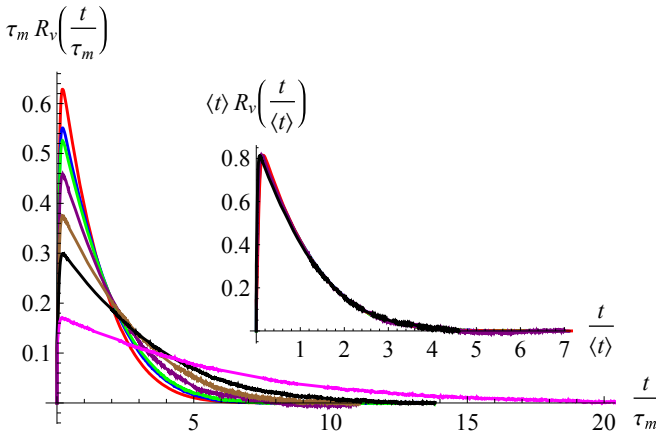
FIG. 12. Main plot: The response function rescaled with the theoretically predicted time scale \tau_m . Velocities from top to bottom are v = 0 (red), v = 0.3 (blue), v = 0.5 (green), v = 1 (violet), v = 1.5 (brown), v = 2 (black) and v = 3 \approx f_c (magenta). Inset: Scaling collapse for the velocities v \leq 2 , using the measured time scale \langle t \rangle instead of \tau_m for the rescaling. (DNS, \delta u = 10^{-6} , \delta t = 10^{-4} , N = 10^7 ).
