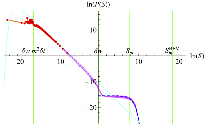
FIG. 13. Avalanche-size distribution P(S) for a particle with forces given by Eq. (6). The theoretical curves are the kicked ABBM model as given by Eq. (46) (cyan dotted), and the DPM as given by Eq. (62) (blue, dashed). INS, m^2 = 10^{-4} , \delta w = 1 , \delta t = 10^{-4} , S_m := \langle S^2 \rangle / (2 \langle S \rangle) = 2408.89 , \rho_m = 2329.95 , N = 10^8 .
