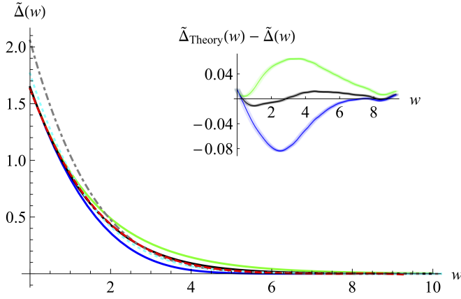
FIG. 17. Convergence of the measured \tilde{\Delta}(w) for m^2 = 10^{-2} (gray, dot-dashed), m^2 = 10^{-3} (cyan, dotted) and m^2 = 10^{-4} (red, dashed). This is compared to three theoretical curves: an exponential function with the same slope at w = 0 (green, top curve), Eq. (92) (black, middle curve), and the 1-loop FRG-result (blue, bottom curve), see Eqs. (4.5) and (4.11) of [23]. The inset shows the difference of the measured \tilde{\Delta}(w) at m^2 = 10^{-4} , and the theoretical curves in their respective colors, together with error bars at a 99% confidence level.
