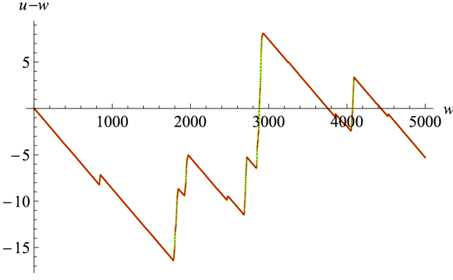
FIG. 3. u_w - w for \delta t = 10^{-4} , v = 0.1 , m^2 = 0.1 , INS. See section B for implementation details. Red points are data points equally spaced in time, the green line between them is an interpolation.
