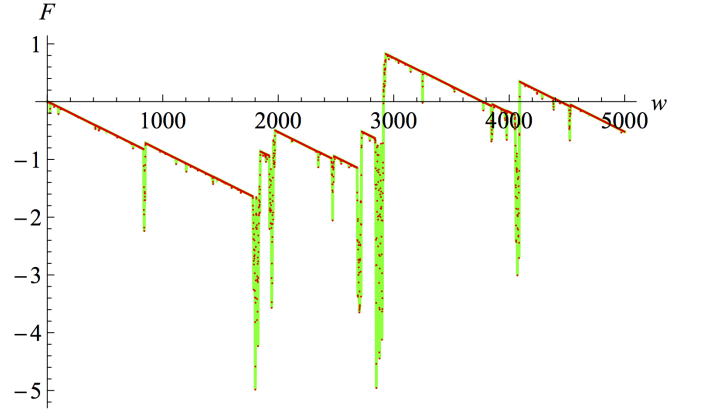
FIG. 5. F(w) with the same parameters as in Fig. 3.
