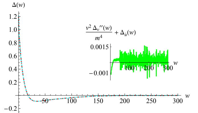
FIG. 16. Numerical test of Eq. (88) for m^2 = 10^{-2} , v = 0.5 . Plotted is \Delta_{\dot{u}}(w) (cyan, dotted) and -\frac{v^2}{m^4} \Delta_v''(w) (red, dashed). The inset shows the difference. (DNS, \delta u = 0.01 , \delta t = 10^{-4} , N = 10^8 ).
