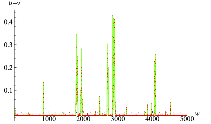
FIG. 4. \dot{u}(w) - v with the same parameters as in Fig. 3.
