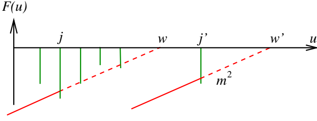
FIG. 1. Geometric solution to find u_w as a function of w for the DPM model of [33].
