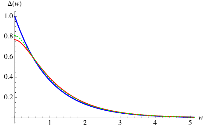
FIG. 2. \Delta(w) = e^{-w} (blue solid), and the finite-velocity correlator (25) (red) for \tau v = 0.3 , compared to the boundary-layer approximation (27) (green dotted).
