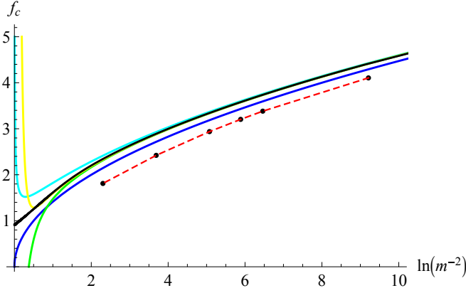
FIG. 6. The critical force f_c as a function of m . Thick black: the results of the integral (68). The small- m expansion is in blue, cyan, green, and yellow. The data points are from our numerical simulation. DNS, \delta u = 10^{-2} , \delta t = 10^{-4} , N = 3 \times 10^6 .
