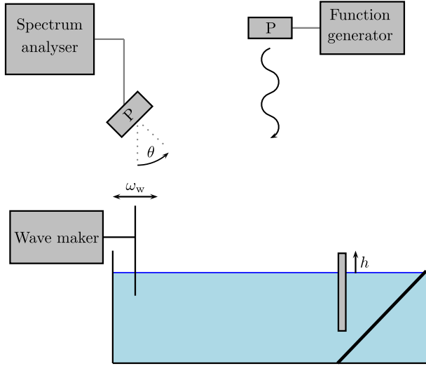
FIG. 4. Experimental setup for the measurement of the reflection coefficient. P stands for piezoelectric transducer and the distance between the vertical barrier and the edge of the basin is longer than sketched here.
