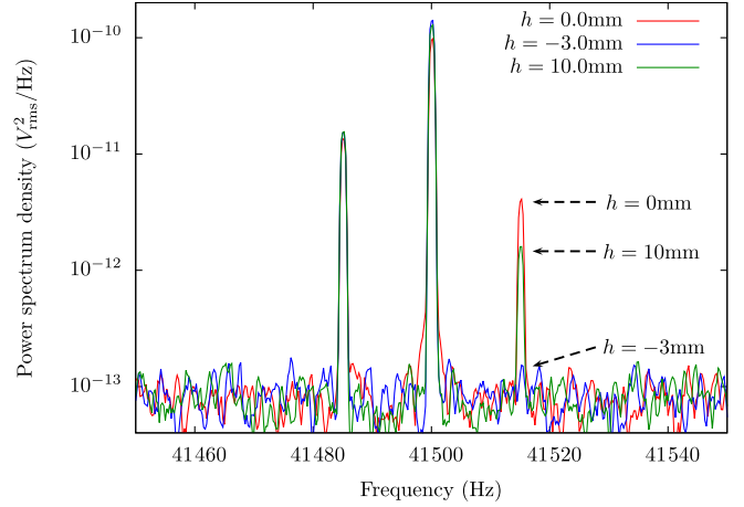
FIG. 5. Typical acoustic spectra for different elevations.
