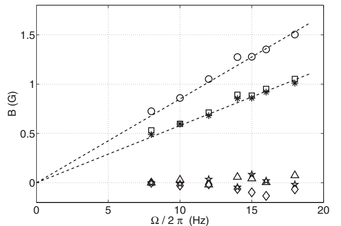
FIG. 3. Evolution with the rotation frequency of the increments of the mean values of components \langle B_i \rangle(\Omega/2\pi) - \langle B_i \rangle(\Omega/2\pi = 8 \text{ Hz}) , \langle B_x \rangle ( \diamond ), \langle B_y \rangle ( \triangle ), \langle B_z \rangle ( \star ), and standard deviations, B_{xrms} ( \circ ), B_{yrms} ( \square ), B_{zrms} ( \ast ). Linear fits of the standard deviations with dashed lines.
