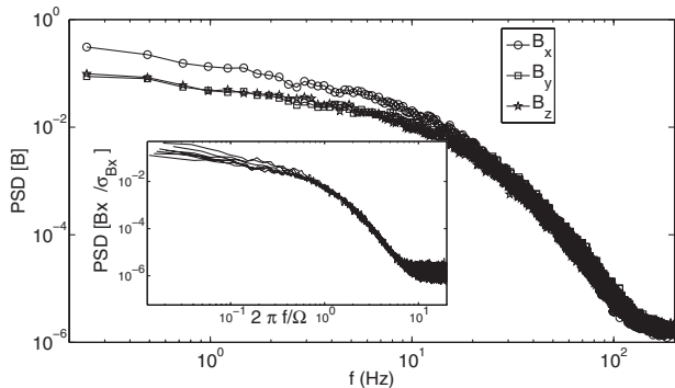
FIG. 5. Power spectra of the fluctuations of each component of the induced magnetic field for \Omega/2\pi = 15 Hz. B_x ( \circ ), B_{yrms} ( \square ), B_{zrms} (*). Inset: power spectra of the fluctuations of B_x normalized by its standard deviation \sigma_{Bx} vs 2\pi f/\Omega for \Omega/2\pi = 8, 10, 12, 14, 15, 16, 18 Hz.
