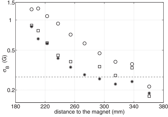
FIG. 4. Spatial decay of the induced magnetic field rms fluctuations in space. B_{xrms} ( \circ ), B_{yrms} ( \square ), B_{zrms} (*). Disk rotation frequency, \Omega/2\pi = 15 Hz. The horizontal dashed line corresponds to 0.26 G, i.e., twice the standard deviation of the fluctuations induced by the Earth magnetic field alone.
