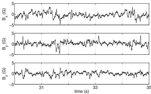
FIG. 2. Direct time recordings of the fluctuations of the induced magnetic field components measured by the first probe ( P in Fig. 1), 200 mm away from the magnet. Disk rotation frequency, \Omega/2\pi = 15 Hz.
