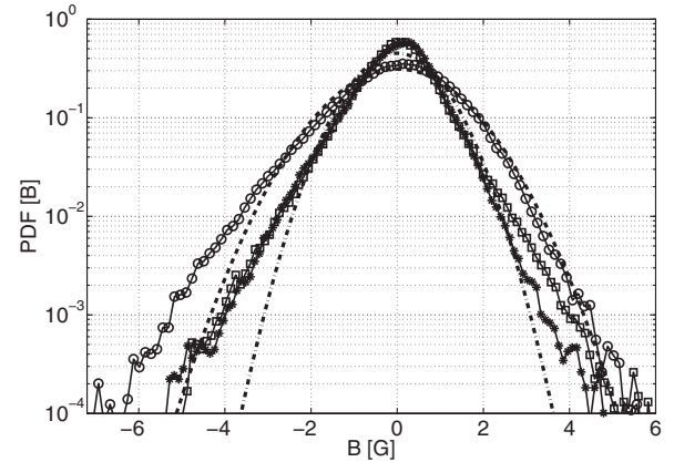
FIG. 6. PDF of the fluctuations of the induced magnetic field: B_x ( \circ ), B_y ( \square ), B_z (*). Disk rotation frequency, \Omega/2\pi = 15 Hz. The dashed (dash-dotted) curve is a Gaussian with standard deviation equal to the one of B_x ( B_y or B_z ).
