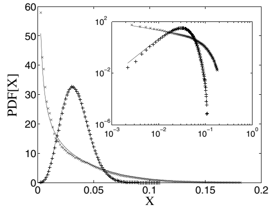
FIG. 2. PDF of the solutions of (1) with the noise (6). The symbols ( \times ) and ( + ) correspond, respectively, to the parameters used in Figs. 1(a) and 1(b). The full lines are the corresponding predictions given by (4). Same figure in inset using log-log scale.
