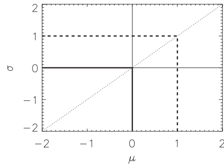
FIG. 7. Stability (solid line) and on-off intermittency boundaries (dashed line) for the scalar noise that does not break the continuous symmetry [Eq. (22)] with \phi = 0 .
