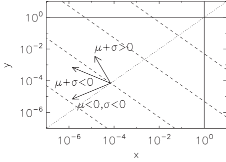
FIG. 15. Diffusion lines in log-log scale for the noise term that breaks symmetry [Eq. (30)] with \phi=0 .
