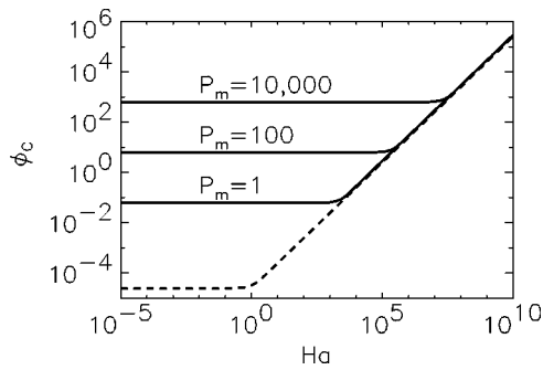
FIG. 8. Upper bound on dissipation rate for Couette flow as a function of Ha for different Prandtl numbers. The dashed line shows the dissipation of the laminar solution. The Reynolds number Re=10\,000 for all cases.
