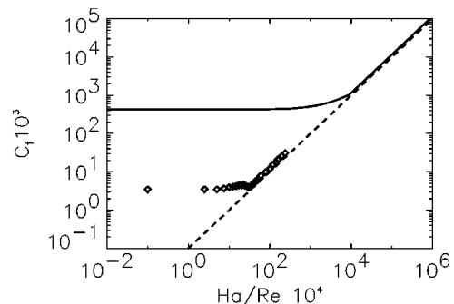
FIG. 15. Drag coefficient C_f as a function of Ha/Re . The diamonds are experimental data from Ref. 5 for Re = 5 \times 10^5 . The dashed line is the drag coefficient for the laminar solution and the solid line is the upper bound.
