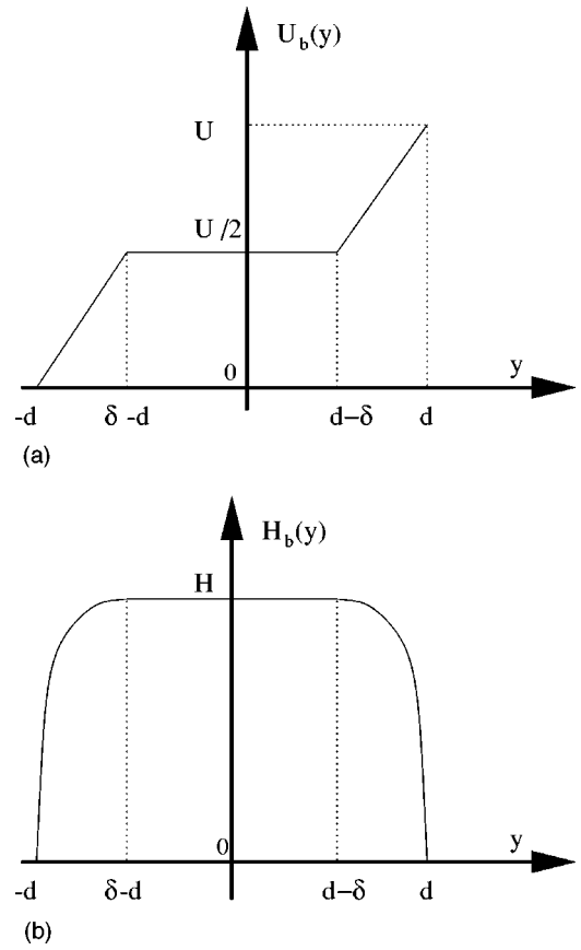
FIG. 7. Panel (a) shows the background field U_b(y) and panel (b) shows H_b(y) , where H := B_0 \delta / 4\eta .
