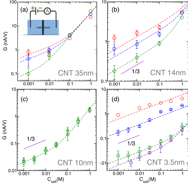
FIG. 1. Conductance G = I/\Delta V measured inside single carbon nanotubes with various geometrical characteristics and pH . (a) \{R, L\} = \{35 \text{ nm}, 1500 \text{ nm}\} , pH = 6, 9, 10 from bottom to top; (b) \{R, L\} = \{14 \text{ nm}, 2000 \text{ nm}\} , pH = 6, 9, 10 from bottom to top; (c) \{R, L\} = \{10 \text{ nm}, 2500 \text{ nm}\} , pH = 4 ; (d) \{R, L\} = \{3.5 \text{ nm}, 3000 \text{ nm}\} , pH = 4, 6, 8, 10 from bottom to top. The dashed lines are predictions according to the model in the text, G = 2e^2\mu(\pi R^2/L)\sqrt{\rho_s^2 + \Sigma^2/R^2} , with a surface charge scaling with salt concentration C_{\text{salt}} as \Sigma \propto C_{\text{salt}}^{1/3} ( C_{\text{salt}} in \text{Mol L}^{-1} and \rho_s = 6.0210^{26} \times C_s the numerical density in \text{m}^{-3} ). See text and Supplemental Material [15] for details.
