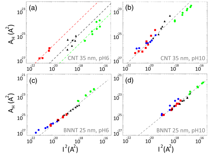
FIG. 3. Evolution of the parameter A_H with the dc ionic current I (log-log scales). The experiments have been performed on CNT with \{R, L\} = \{35 \text{ nm}, 1500 \text{ nm}\} (a) and (b) and BNNT with \{R, L\} = \{25 \text{ nm}, 500 \text{ nm}\} (c) and (d), for different values of pH [ pH6 , (a) and (c) and pH10 , (b) and (d); see Supplemental Material [15] for the curves at pH9 ]. The colors of the symbols correspond to various KCl concentration: 10^{-3} \text{ M} (blue), 10^{-2} \text{ M} (red), 10^{-1} \text{ M} (black), 1 \text{ M} (green). The dashed lines have a slope 1 in log-log scales, highlighting the linear dependence of A_H with I^2 .
