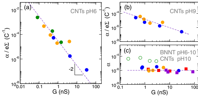
FIG. 4. Collapse of the noise amplitude rescaled by surface charge, \alpha/e\Sigma , as a function of the conductance G . The symbols are CNT with \{R, L\} = \{35 \text{ nm}, 1500 \text{ nm}\} (blue); CNT with \{R, L\} = \{14 \text{ nm}, 2000 \text{ nm}\} (orange); CNT with \{R, L\} = \{7 \text{ nm}, 1000 \text{ nm}\} (green). (a) Results at pH6 . The dashed line has a slope equal to -2 , \alpha/\Sigma \propto 1/G^2 . (b) Results at pH9 . The dashed line has a slope equal to -1.2 , \alpha/\Sigma \propto 1/G^{1.2} . (c) \alpha versus conductance for the three CNTs at pH10 and BNNT with \{R, L\} = \{25 \text{ nm}, 500 \text{ nm}\} at pH6 (red) and pH10 (violet).
