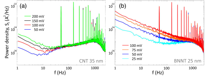
FIG. 2. Noise current power spectra for CNT with \{R, L\} = \{35 \text{ nm}, 1500 \text{ nm}\} (a) and BNNT with \{R, L\} = \{25 \text{ nm}, 500 \text{ nm}\} (b), measured at pH6 and at salt concentration equal to 1 \text{ M} , for different applied voltage. Peaks in the noise at harmonics of 50 \text{ Hz} are due to ac electric supply grid.
