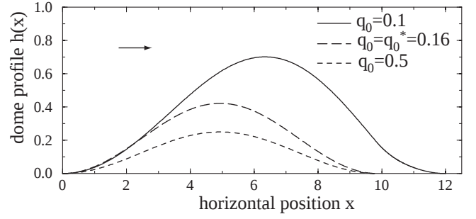
Fig. 8. Shape of the dome solution for different values of the sand flux q_0 , for \alpha = 1 and \beta = 4 . Note the asymmetry upwind/downwind of the low flux dome. For clarity the scale of the vertical axis is much larger than that of the horizontal one.
