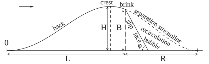
Fig. 2. The sand transport increases on the back of the dune which is thus eroded. The sand is deposited at the brink and is redistributed along the slip face by avalanches. It can be assumed that the slip face is always at the repose angle \varphi . At the brink, the turbulent boundary layer separates from the dune, enclosing a recirculation bubble. In the absence of better approximations, the separation streamline is assumed to extend the dune profile and to reattach the ground smoothly. By definition, L is the distance between the foot of the dune ( x = 0 ) and the brink x = L , H is the height of the highest point of the dune (crest) and B is the dune height at the brink. H and B may coincide or not.
