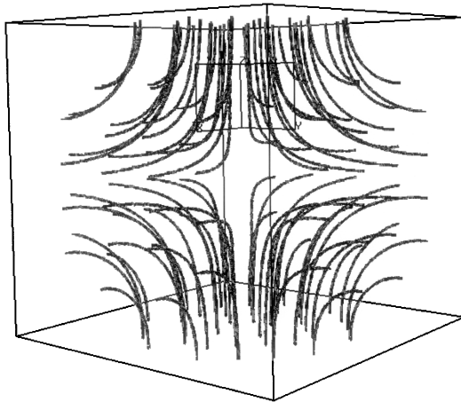
FIG. 1. Three-dimensional visualization of the vector field \nabla \times (\rho \mathbf{v}) for the Taylor-Green flow at time t = 0 with coherence length \xi = 0.1/(8\sqrt{2}) , sound velocity c = 2 , and resolution N = 512 in the impermeable box [0, \pi] \times [0, \pi] \times [0, \pi] . The visualization is obtained by drawing the 30 000 vectors of highest norm.
