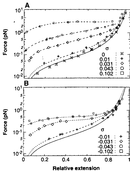
Fig. 2. Force versus relative extension (43) curves for a single torsionally constrained molecule at various degrees of supercoiling ( \sigma ). (A) \sigma = 0, 0.01, 0.031, 0.043, and 0.102 . (B) \sigma = -0.01, -0.031, -0.043, and -0.102 . The full line is the theoretical prediction for a wormlike chain with a persistence length of 53 nm (25). The dashed lines are polynomial fits, as a guide to the eye, except for \sigma = \pm 0.01 , where a wormlike chain with a persistence length of 35 nm was fitted. Notice that at low forces ( F < 0.3 pN) the curves for positive and negative supercoiling are similar. However, at forces greater than \sim 0.45 pN, there is a significant difference between the two curves as the underwound molecule undergoes a transition to an extended state whose elastic behavior is similar to that of the \sigma = 0 torsionally relaxed one. Notice also the similar sharp transition for \sigma = 0.102 at F \sim 3 pN. For short relative extensions ( < 10\% ), the force measurements are unreliable because of interactions with the surface and poor Brownian statistics.
