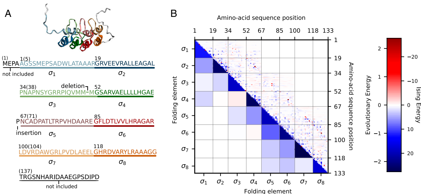
Fig. 1. Model definition. (A) Folding elements are 18- and 15-residue repeat subunits, as highlighted on the p16 sequence. They correspond to first and second alpha-helix of each repeat, respectively, as colored on the Protein Data Bank (PDB) structure. (B) Double energy heat map for p16. Evolutionary residue pairwise couplings J_{ab}(\sigma_a, \sigma_b) on the upper side and single-residue contributions h_a(\sigma_a) on the diagonal were added according to folding elements and rescaled to define Ising energies \epsilon^i(\sigma_j) and \epsilon^s(\sigma_j, \sigma_k) on the lower side. Blue (red) dots represent evolutionary (un)favorable pairs and positions. On the lower side, almost all internal and interaction folding energies are favorable; hence, they are blue.
