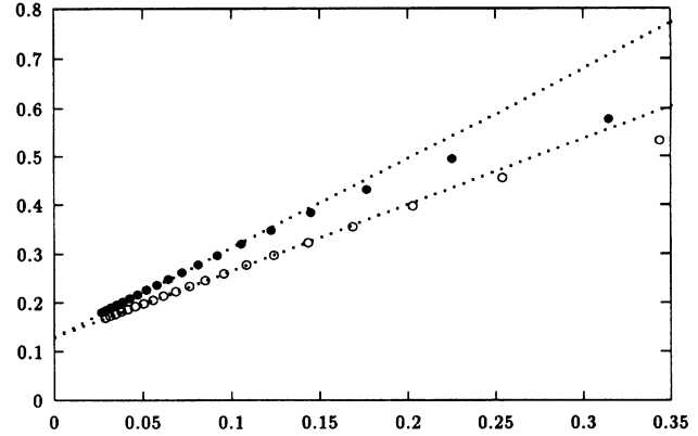
FIG. 2. The masses \tilde{m}_L = 1/\tilde{\xi}_L (empty dots) and m_L = 1/\xi_L (full dots) plotted vs the “finite-size” factors \exp(-L/\tilde{\xi}_L) and \exp(-L/\xi_L) , respectively. The dashed lines are the best linear fits from the last 12 points (sizes L=9 to L=20 ).
