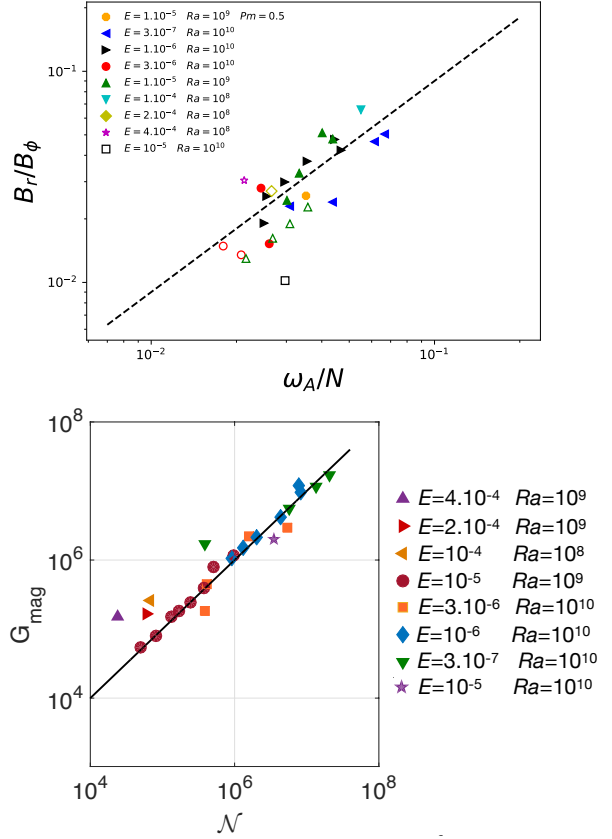
Fig. 6: Top: Dimensionless ratios B_r/B_\phi versus \beta B_\phi / \sqrt{\rho \mu r N} , for the dynamo simulations shown in Petitdemange et al. (2023) and for our additional, highly-stratified model. B_r and B_\phi here are determined by averaging the energy of the m = 0 poloidal and toroidal magnetic fields over space and time (at steady state). Here \beta = 1.8 is a fitting coefficient. Note that empty symbols denote simulations in only weakly supercritical regime (as quantified arbitrarily here by Re/Re_c \leq 5/3 ): because the flow regime remains close to the onset of instability, the relevance of diffusionless scaling is subject to caution. Bottom: Scaling of the dimensionless magnetic torque with Spruit’s diffusionless prediction Eq. 19 (shown with the black line). The data include the simulations shown in (Petitdemange et al. 2023) and an additional, highly-stratified model with Ra = 10^{10} .
