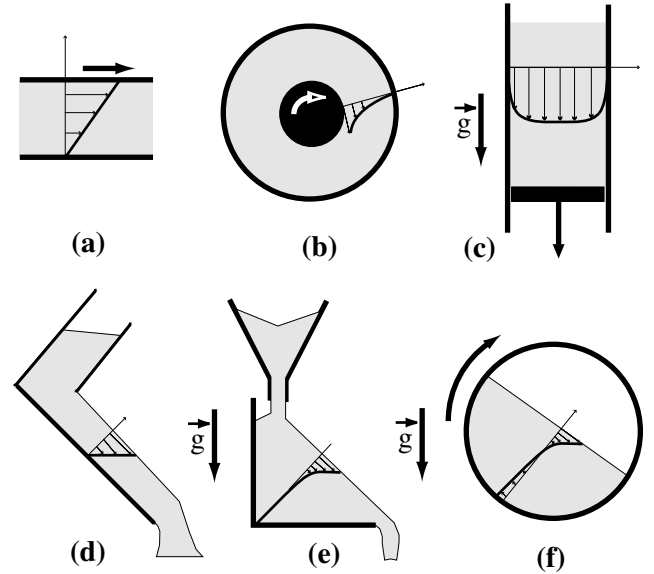
Fig. 1. The six configurations of granular flows: (a) plane shear, (b) annular shear, (c) vertical-chute flows, (d) inclined plane, (e) heap flow, (f) rotating drum.
