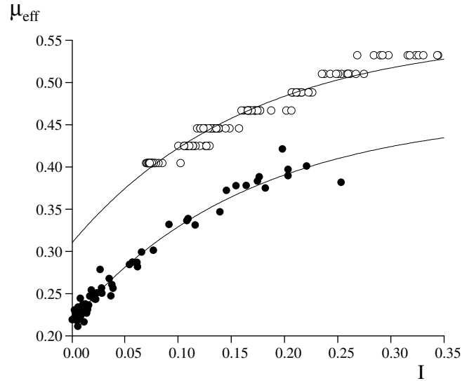
Fig. 8. Comparison of the effective friction function of I in the plane shear ( \bullet ) and the inclined-plane ( \circ ) configurations.
