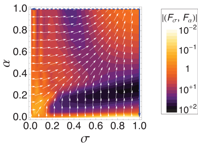
Figure 5 | Map of adiabaticity requirements. Absolute value of the vector (F_\sigma, F_x) is plotted in the coloured map for N = 9 , evidencing the large value of F_x at large \sigma = w^2/(N - 1) and small \alpha , as well as the more favorable condition if one uses a reduction in time of the beam waist. The two paths described in the text give T \sim 40 (solid blue line) and T \sim 20 (dashed blue line). Superimposed white arrows represent the directions of the vector (F_\sigma, F_x) . This plot can serve for conceiving more intricate paths with the help of optimization techniques.
