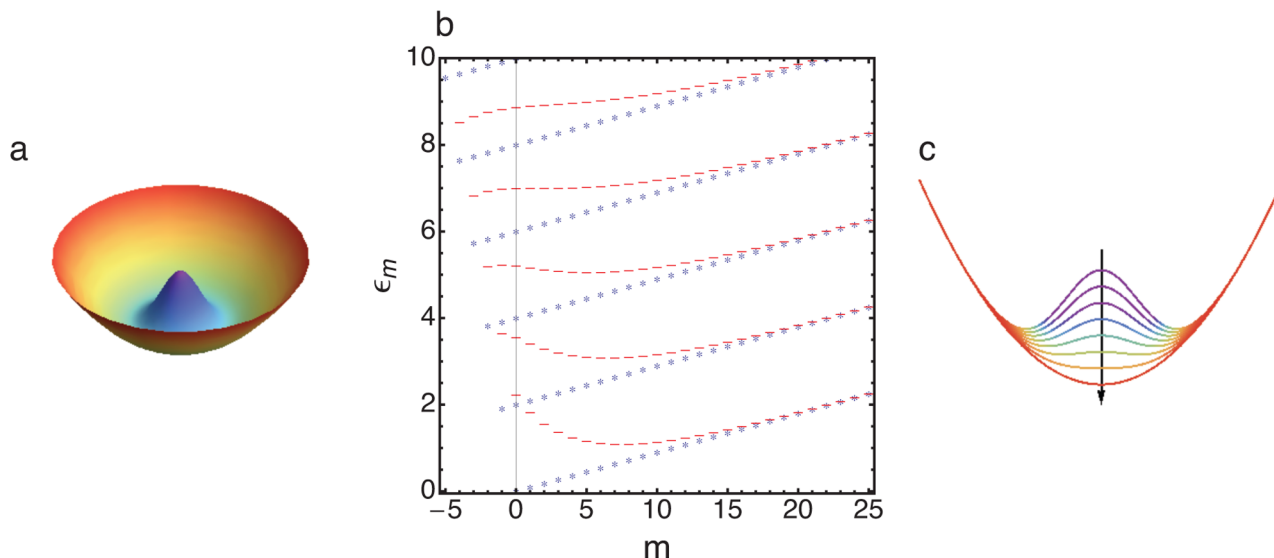
Figure 1 | Mexican hat potential. (a) Bosonic atoms are confined in a combined trap with (i) an isotropic harmonic confinement and (ii) the dipole potential created by a blue-detuned, gaussian laser beam that plugs the trap center and pushes the particles away from this point. The resulting potential exhibits a Mexican-hat shape. (b) Under fast rotation, the single-particle energy spectrum exhibits a Landau Level picture (red dashes), where levels are arranged in quasi-degenerate manifolds as in the case of a purely harmonic trapping (blue asterisks). The level plot has been drawn for \delta = 0.09 , \alpha = 3.0 and w^2 = 8.0 , parameters that we will use in the many-body problem for N = 9 . The single-particle minimum of energy can be adjusted to any desired value on angular momentum by tuning the waist and the power of the plug beam ( m = 8 in the present case). (c) In order to enter FQHE regime of the many-body interacting system, we propose to switch off the plug beam, eventually recovering the usual parabolic form.
