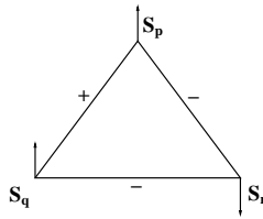
Fig. 8. Spins and couplings for the embassy ball problem.
