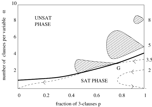
Fig. 4. Phase diagram of 2+p-SAT and dynamical trajectories of DPLL. The threshold line \alpha_c(p) (bold full line) separates sat (lower part of the plane) from unsat (upper part) phases. Extremities lie on the vertical 2-SAT (left) and 3-SAT (right) axis at coordinates (p=0, \alpha_c=1) and (p=1, \alpha_c \simeq 4.3) , respectively. Departure points for DPLL trajectories are located on the 3-SAT vertical axis and the corresponding values of \alpha are explicitly given. Hatched regions symbolize tree trajectories in the unsat region, and dashed curve represent branch trajectories in the sat phase. Arrows indicate the direction of “motion” along branch trajectories parameterized by the fraction t of variables set by DPLL. For small ratios \alpha < \alpha_L , branch trajectories remain confined in the sat phase and end in S of coordinates (1, 0) , where a solution is found. At \alpha_L \simeq 3.003 , the single branch trajectory hits tangentially the threshold line in T of coordinates (2/5, 5/3) ( T depends a priori on the heuristics used, but lies very close to the tricritical point). In the intermediate range \alpha_L < \alpha < \alpha_c , the branch trajectory intersects the threshold line at some point G (that depends on \alpha ). A dense tree then grows in the unsat phase, as happens when 3-SAT departure ratios are above threshold \alpha > \alpha_c \simeq 4.3 . DPLL then reaches back the highest backtracking node in the search tree, that is, the first node when \alpha > \alpha_c , or node G for \alpha_L < \alpha < \alpha_c . In the latter case, a solution can be reached from a new descending branch while, in the former case, unsatisfiability is proven, see Fig. 7.
