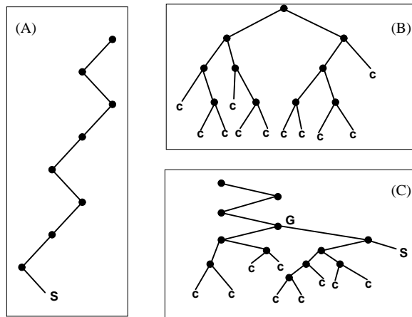
Fig. 7. Types of search trees generated by the DPLL solving procedure. Nodes (black dots) stand for the choices of variables made by the heuristic, and edges between nodes denote the elimination of unitary clauses. A. simple branch : the algorithm finds easily a solution without ever backtracking. B. dense tree : in the absence of solution, the algorithm builds a “bushy” tree, with many branches of various lengths, before stopping. C. mixed case, branch + tree : if many contradictions arise before reaching a solution, the resulting search tree can be decomposed in a single branch followed by a dense tree. The junction G is the highest backtracking node reached back by DPLL.
