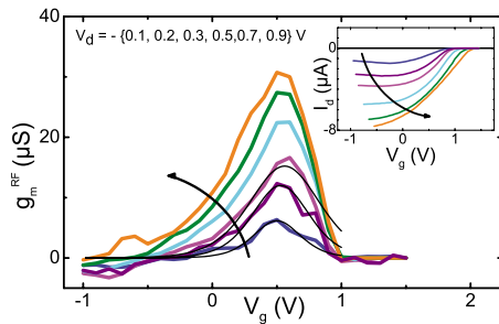
FIG. 2. (Color online) Carbon nanotube transistor characteristics including the dc current (inset) and the rf transconductance g_m^{\text{rf}} measured in the 0–0.8 GHz band (main panel) as function of gate voltage V_g for a representative set of bias voltages increasing according to the arrow. The transconductance maximum for V_g \approx +0.5 V saturates at a large value \approx 30 \mu\text{S} . Low bias data, for V_d = -(100, 200, 300) mV, are fitted with Eq. (2) (solid lines) within a prefactor \approx 0.6 added to account for nonideal ballistic transport above the barrier. The fitting parameter, V_{T_e} = k_B T_e / e\beta \approx (120, 140, 170) \pm 0.01 mV, gives (with \beta = 0.2 ) the thermal energies k_B T_e = (24, 28, 34) meV.
