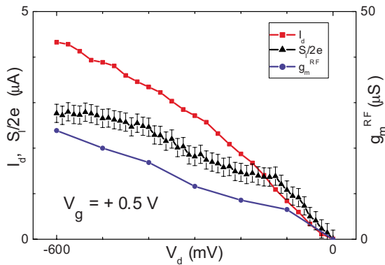
FIG. 4. (Color online) Bias dependence of dc current I_d (squares), rf current noise S_I (triangles), and rf transconductance g_m (circles) at the transconductance maximum ( V_g \sim +0.5 V).
