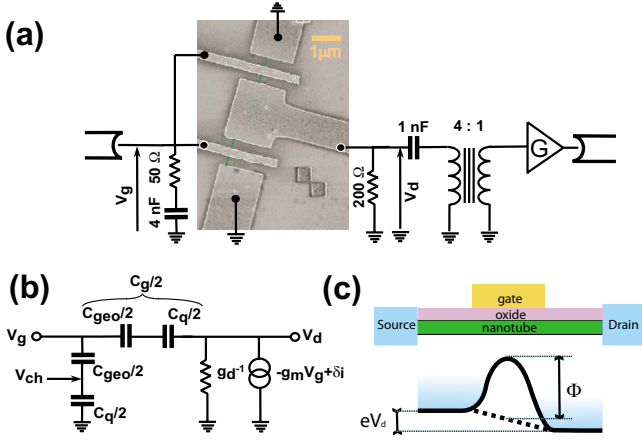
FIG. 1. (Color online) (a) A double gate nanotube transistor embedded in the (4 K) measuring scheme which includes bias resistors, dc blocks and a cryogenic low noise amplifier with a 200:50 \Omega matching transformer. The nanotube of diameter \sim 2 nm, is covered in its middle part by a top gate (length 300 nm) which controls the local barrier. The leads on both sides act as electronic reservoirs. (b) The lumped element description of the nanotube transistor rf response includes the channel resistance g_d^{-1} , the transconductance g_m , the gate capacitance C_g = C_{\text{geo}}C_q/(C_{\text{geo}} + C_q) with its geometrical (respectively quantum) contributions C_{\text{geo}} (respectively C_q ) and the noise current generator \delta i . The channel potential V_{ch} = V_g \times C_g/C_q governs the barrier height \Phi = -e(V_{ch} + \text{const}) which defines the gate coupling coefficient \beta = \partial\Phi/\partial V_g = C_g/C_q . (c) Sketch of the energy profile (solid line) and the electronic distribution (gray scale) of a top-gated nanotube transistor.
