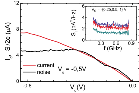
FIG. 3. (Color online) Bias dependence of the dc current and current noise of the nanotube transistor in the metallic state ( V_g \leq 0 ). The intrinsic nanotube shot noise S_I is deduced by fitting the raw noise spectra (inset) with a A + B/f^2 law (solid lines) and subtracting a (B/f^2) Lorentzian tail for the environment noise which contributes below 0.5 GHz and the white noise [ S_I/V_d \approx 1.1 ( \text{pA})^2 \text{V}^{-1} ] of the 200 Ohm bias resistance, which is independently measured at the pinch-off. Accurate shot noise data, in the 0.1–0.8 GHz band, are plotted in the main panel as function of bias voltage for comparison with dc current. We observe full shot-noise ( S_I/2e \approx I_d ) for V_d > -0.4 V and a noise saturation for V_d < -0.4 V.
